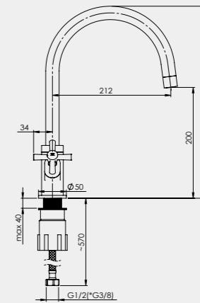
VALENCIA-33 Kitchen faucet 1/2-VL30008 | 3/8-VL30108
