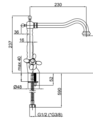
TOSCANA-33 Kitchen faucet 1/2-M8L006 | 3/8-M8L106
