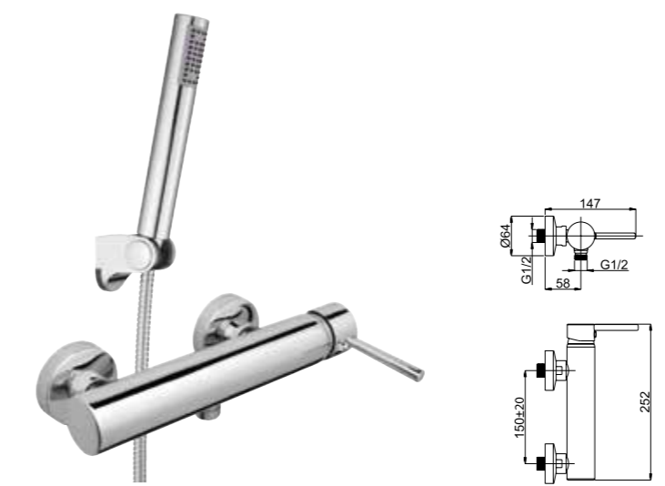
ULTRA-12/K Shower faucet with handshower U20K08 | U20KL08 (Lux)* *Lux type eccentrics art. 636602, page 167.
