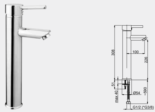
ULTRA-18/D Washbasin faucet 1/2-UD0008 | 3/8-UD0108
