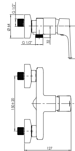
MODENA-12/K Shower faucet with handshower MD20K08 | MD20KL8 (Lux)*
