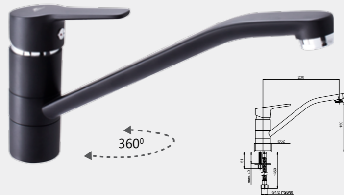
UNO-20 (BK) Kitchen faucet 1/2-N00061 | 3/8-N00161
